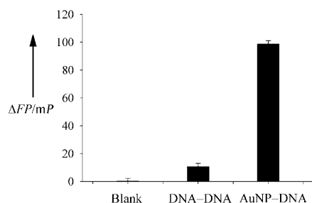
Figure 1. Fluorescence polarization changes upon addition of \text{Hg}^{2+} ions at a concentration of 1.0 \mu\text{M} . A blank (probes A and B without \text{Hg}^{2+} ions) was used as a control reference.
